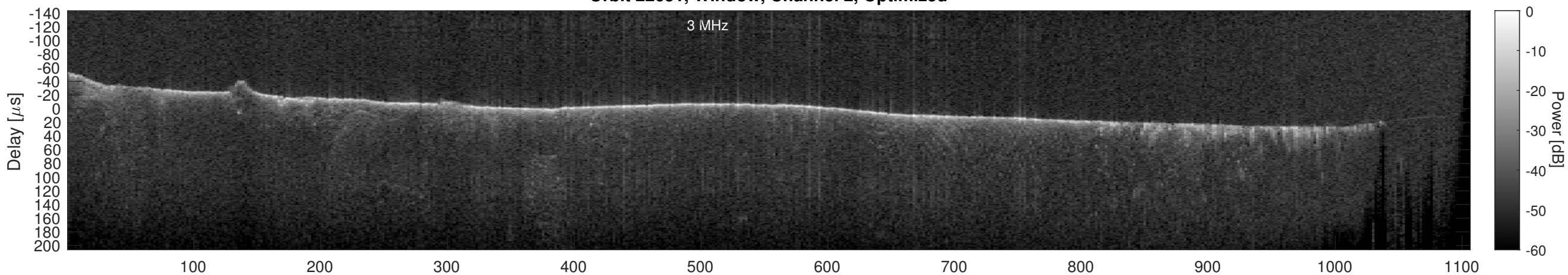
Orbit 22651, Cluttergram
