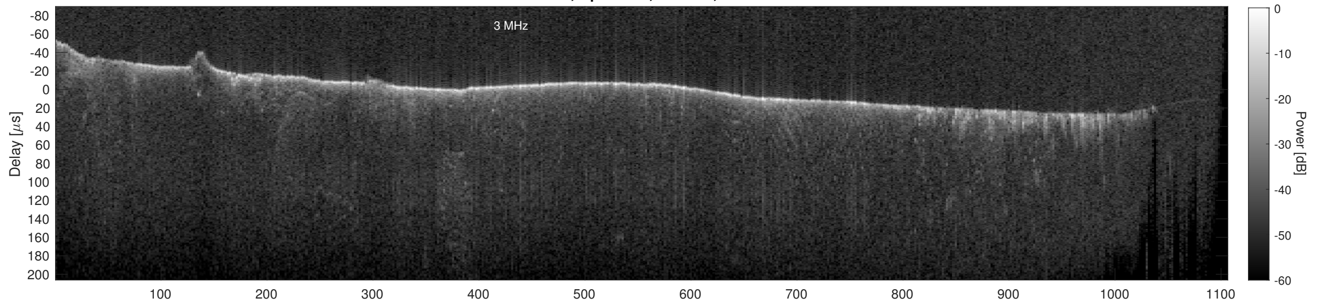
Orbit 22651, Cluttergram
