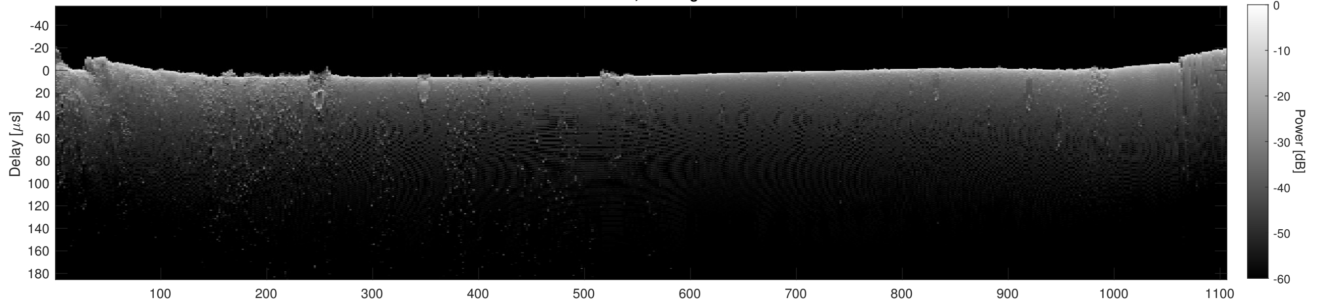
Orbit 22655, Cluttergram
