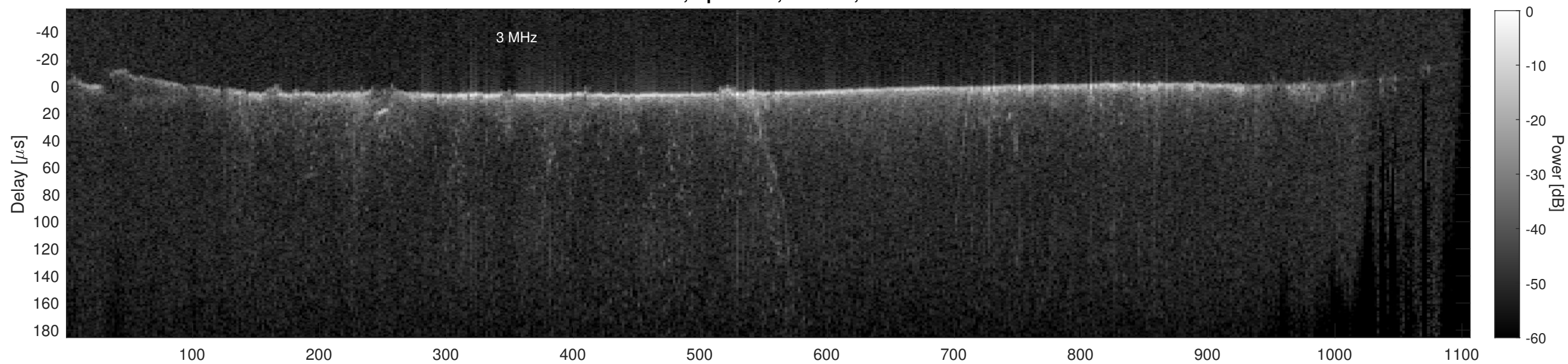
Orbit 22655, Cluttergram
