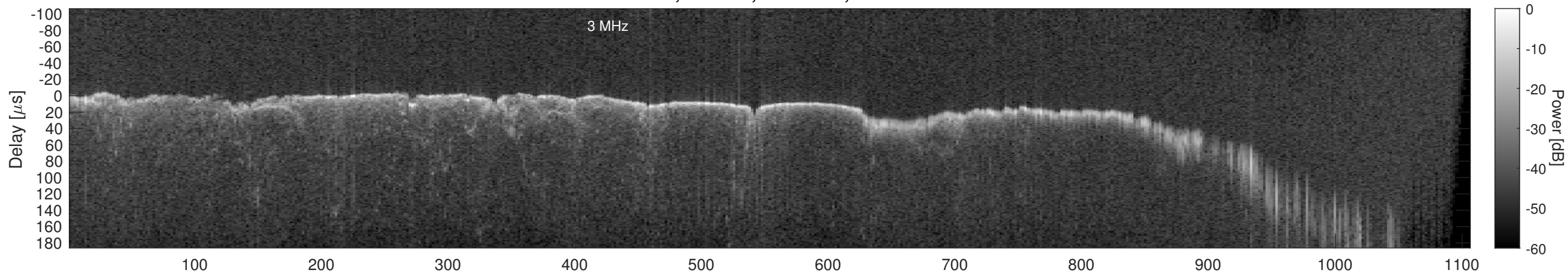
Orbit 22657, Window, Channel 2, Chapman
