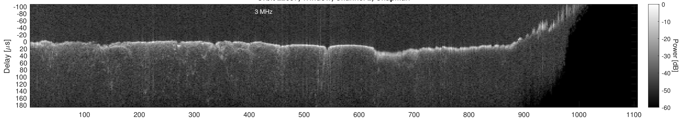
Orbit 22657, Window, Channel 2, Optimized
