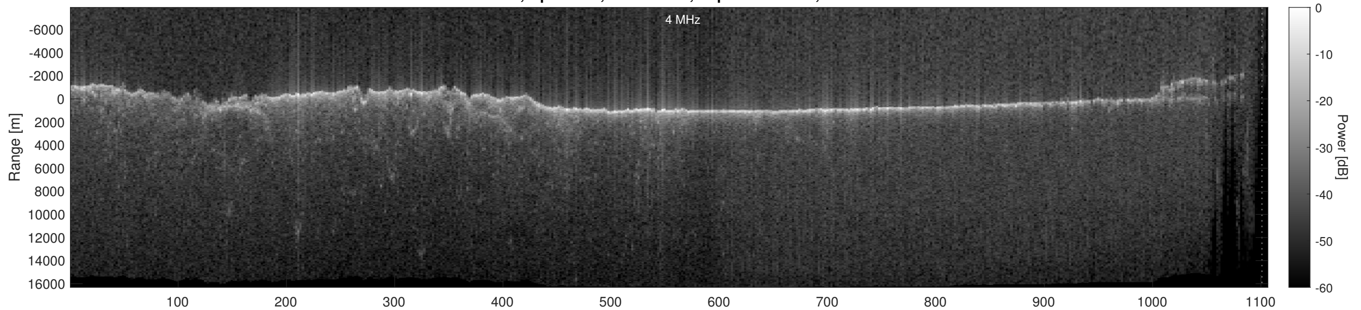
Orbit 22657, Optimized, No Window, Depth-Corrected, Channel 2
