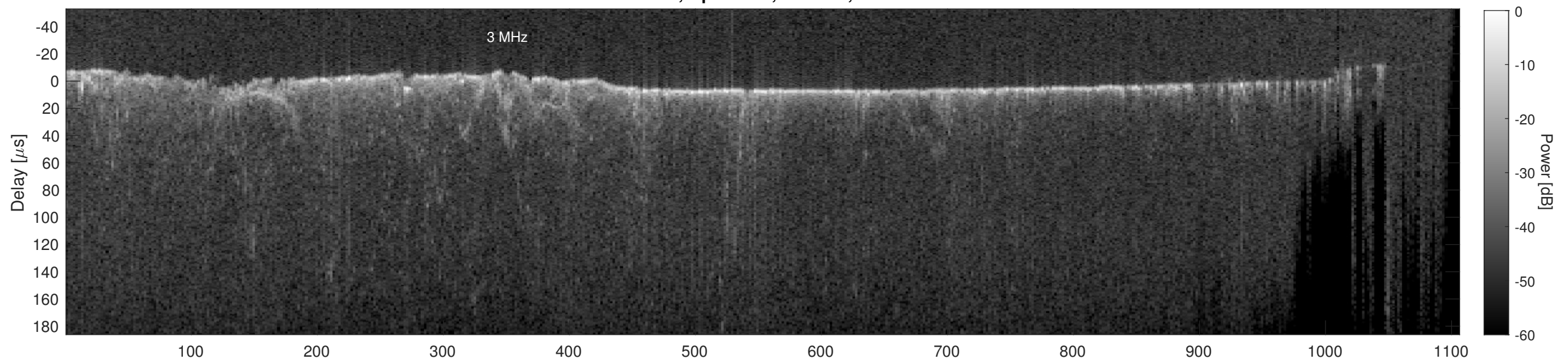
Orbit 22657, Cluttergram
