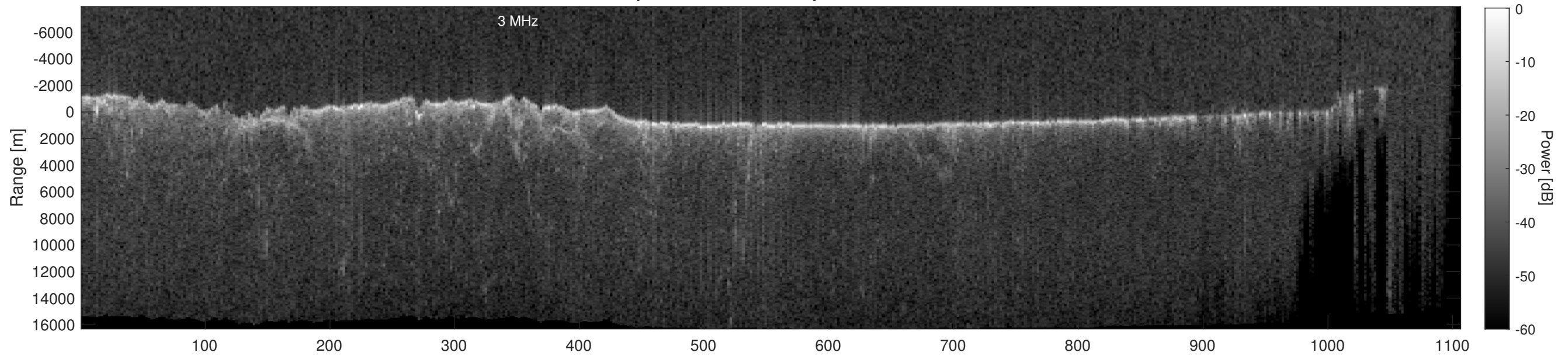
Orbit 22657, Depth-Corrected Cluttergram
