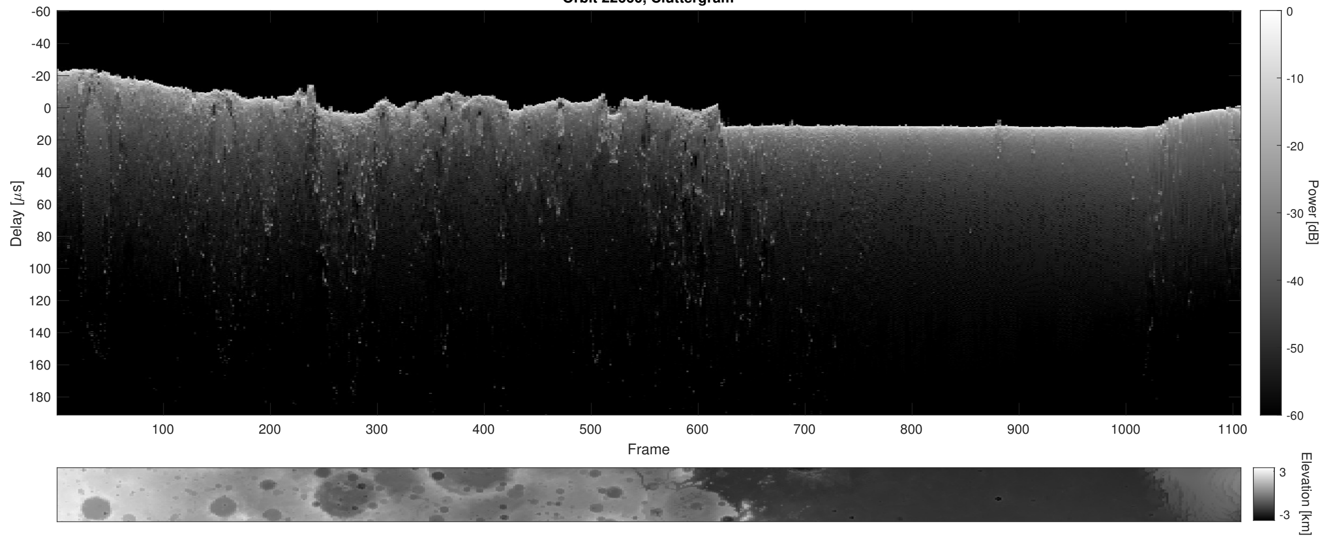
Orbit 22660, Cluttergram
