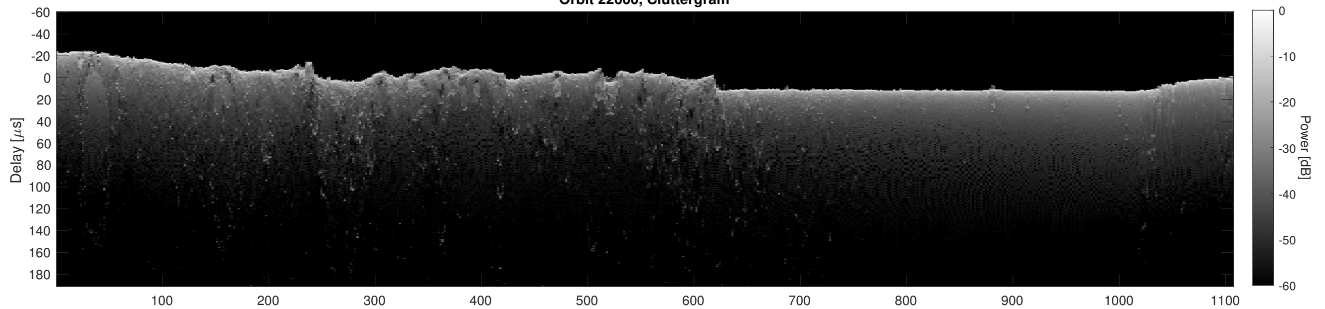
Orbit 22660, Cluttergram
