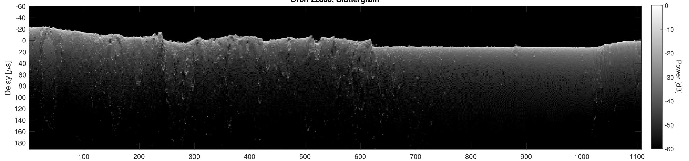
Orbit 22660, Cluttergram
