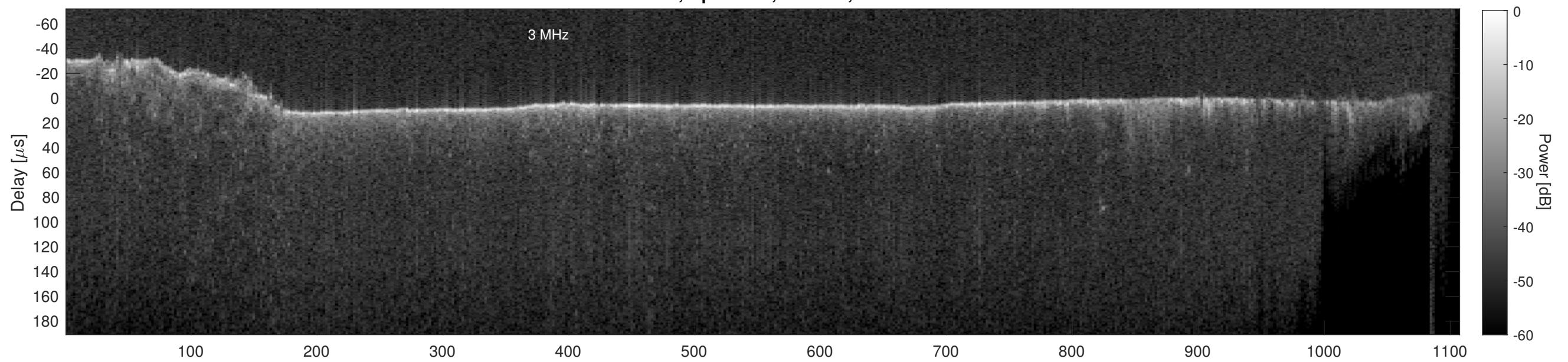
Orbit 22663, Cluttergram
