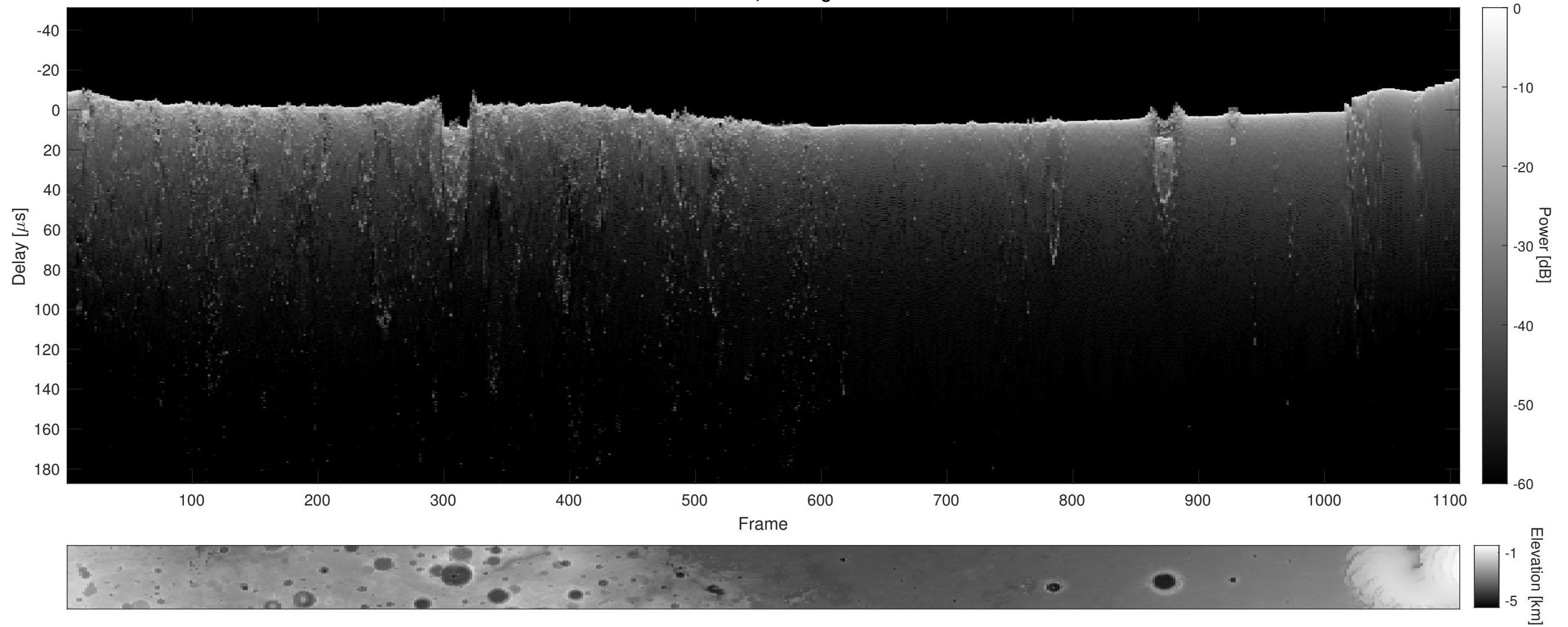
Orbit 22664, Cluttergram
