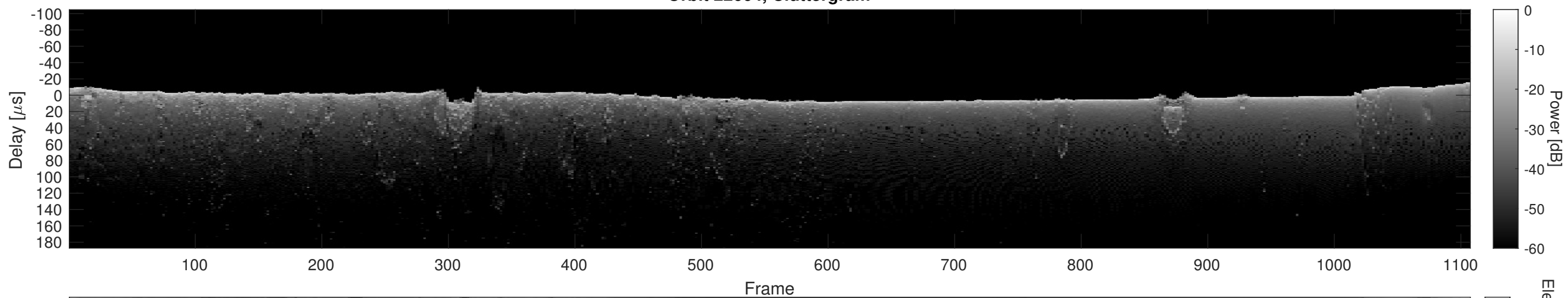
Orbit 22664, Cluttergram
