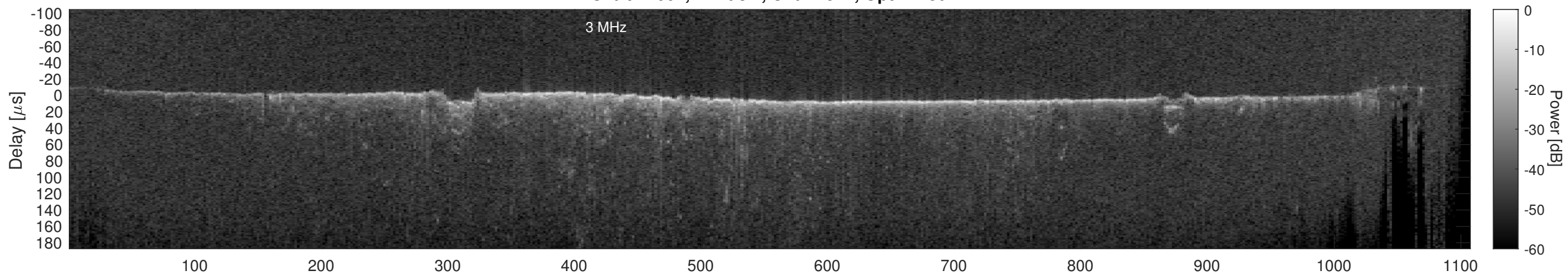
Orbit 22664, Cluttergram
