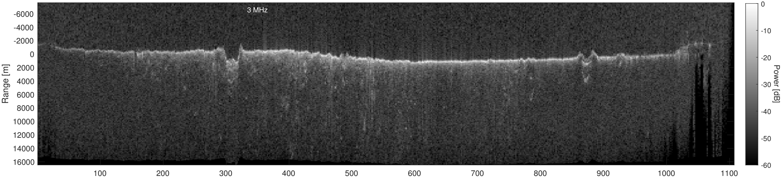
Orbit 22664, Depth-Corrected Cluttergram
