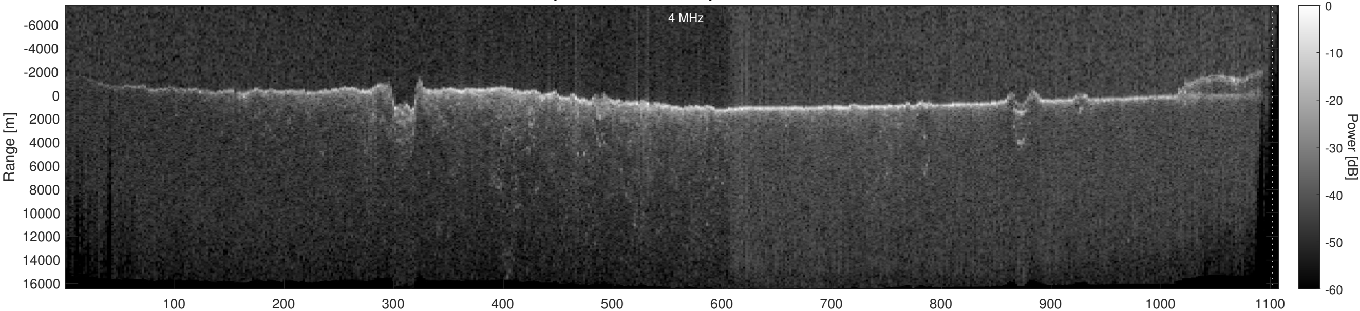
Orbit 22664, Optimized, Window, Depth-Corrected, Channel 2
