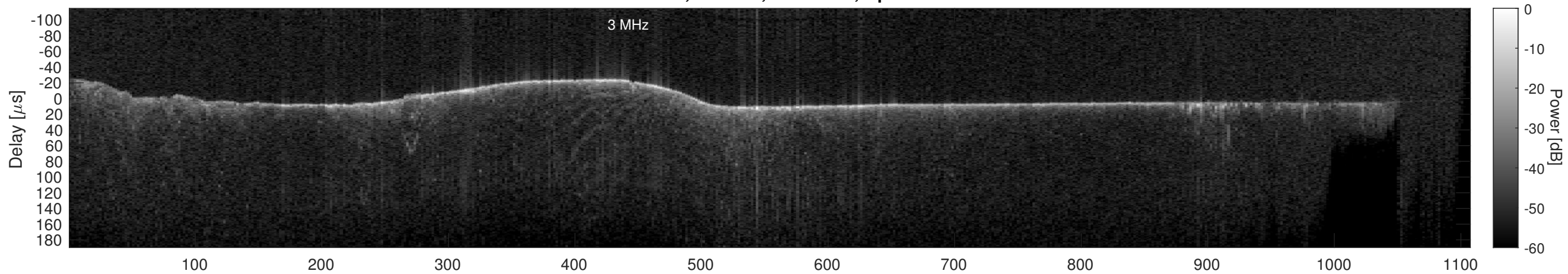
Orbit 22666, Cluttergram
