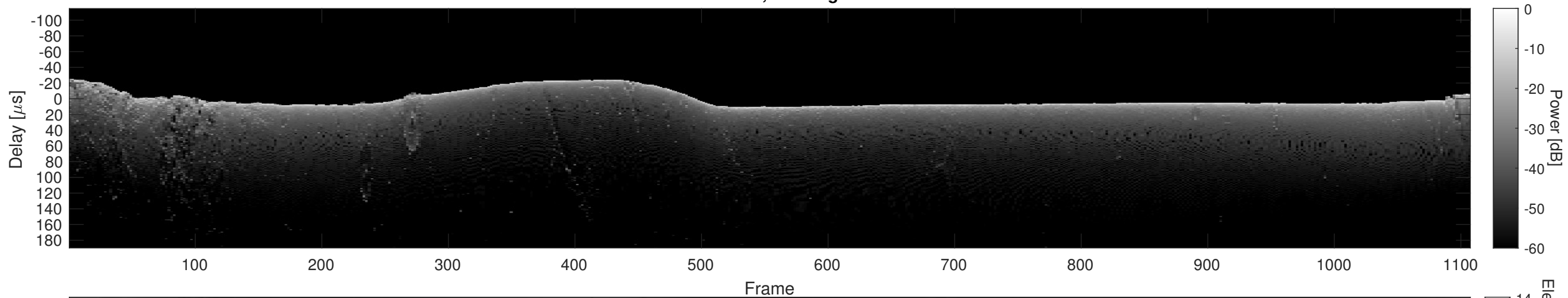
Orbit 22666, Cluttergram
