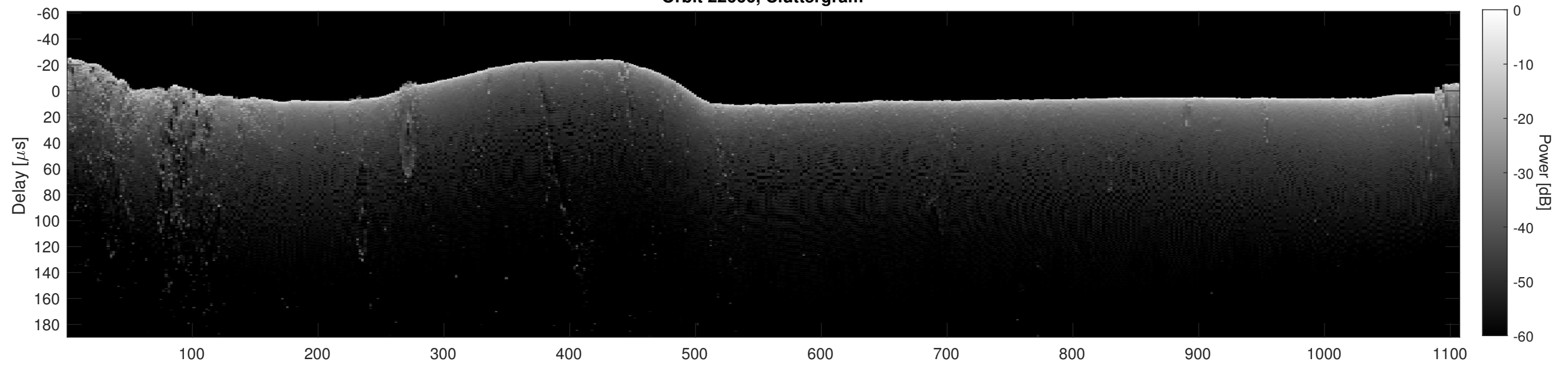
Orbit 22666, Cluttergram
