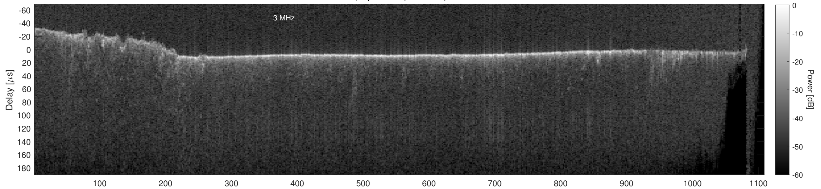
Orbit 22670, Cluttergram
