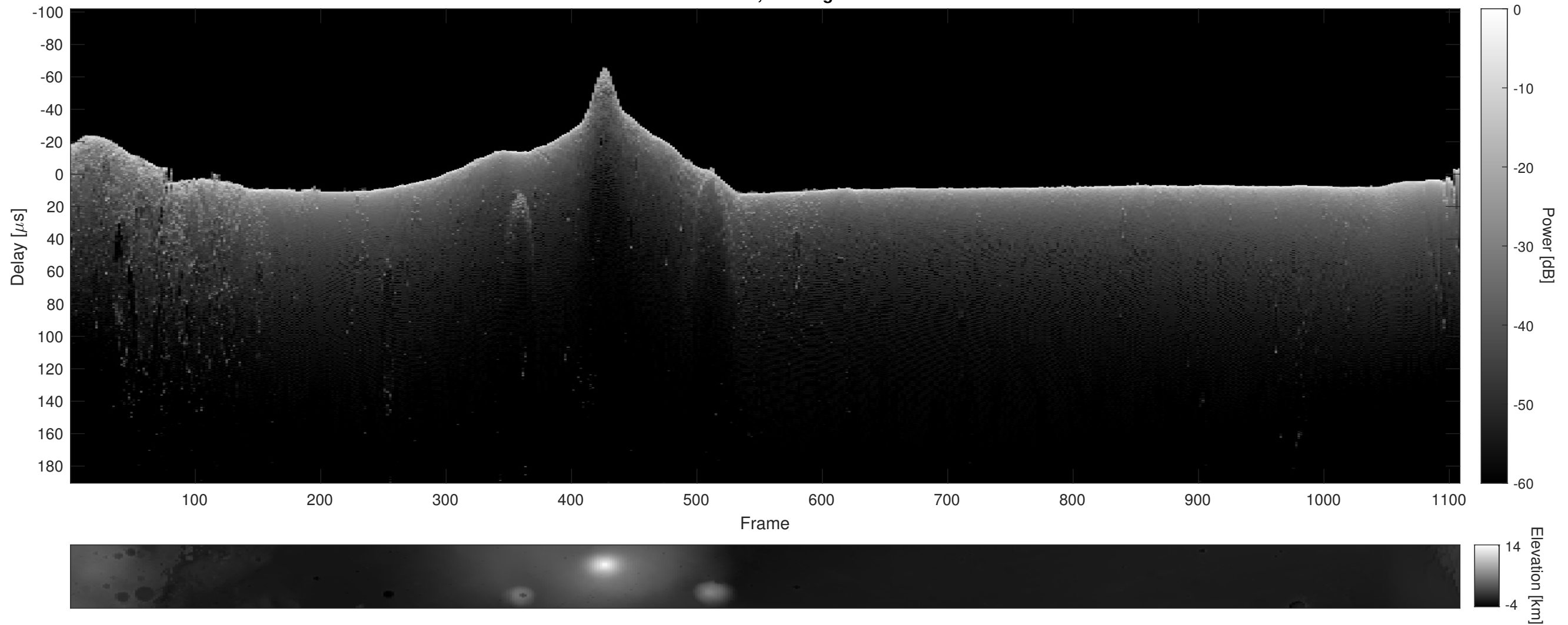
Orbit 22673, Cluttergram
