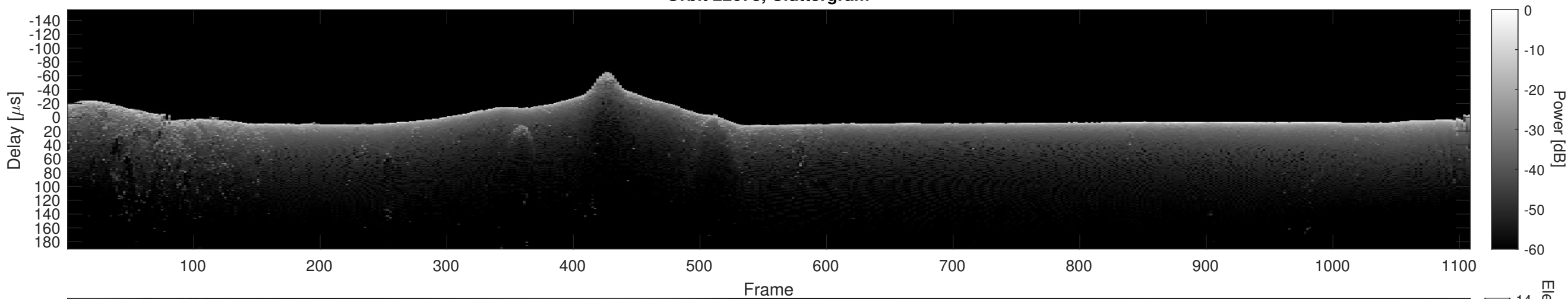
Orbit 22673, Cluttergram
