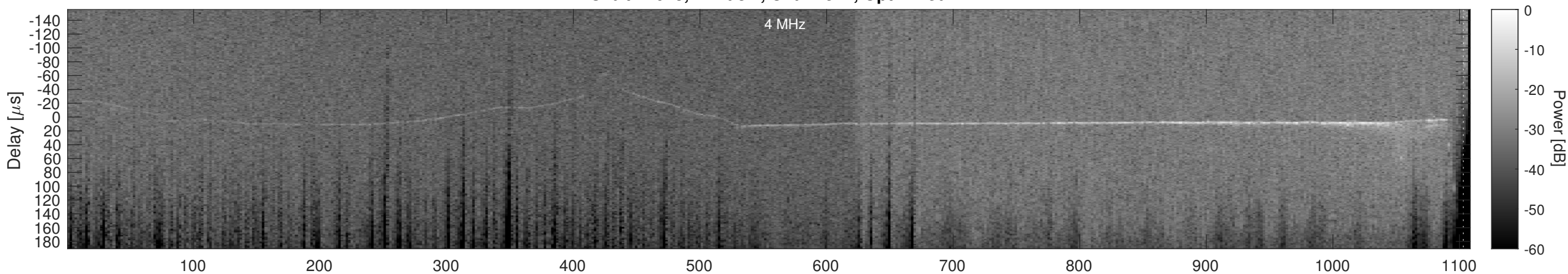
Orbit 22673, Cluttergram
