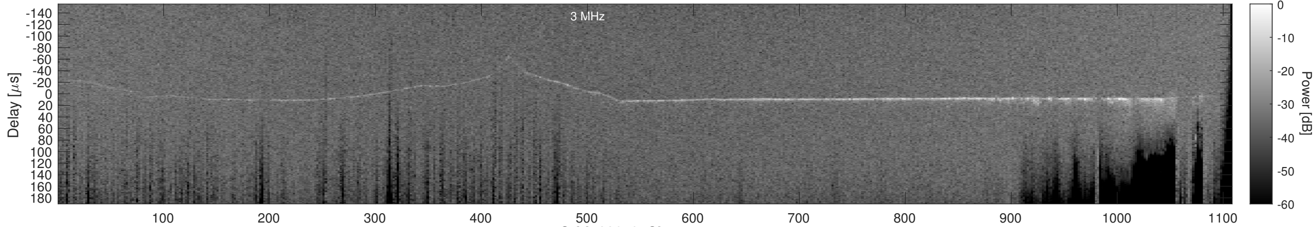
Orbit 22673, Cluttergram
