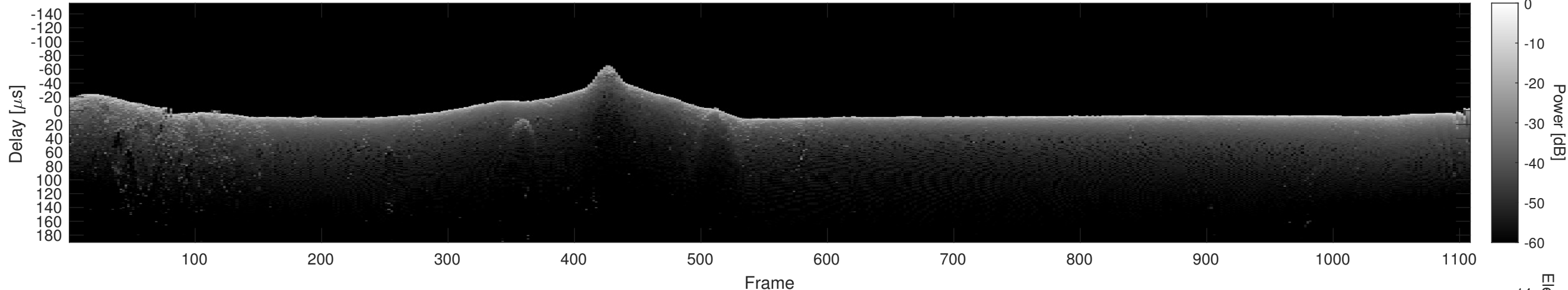
Orbit 22673, Cluttergram
