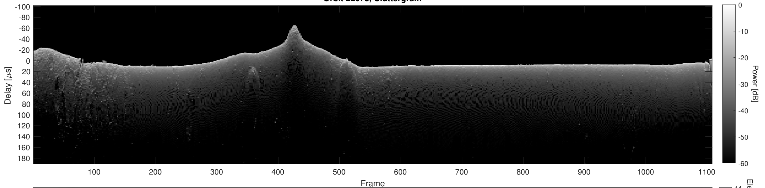
Orbit 22673, Cluttergram
