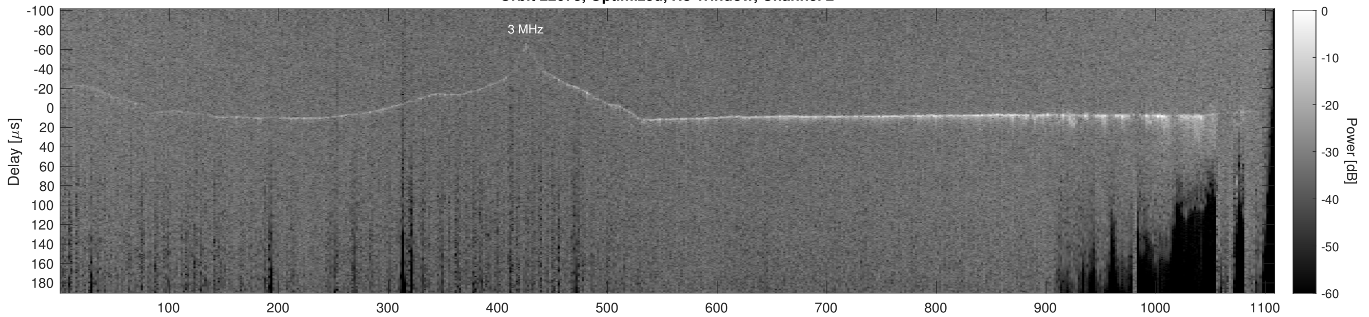
Orbit 22673, Cluttergram
