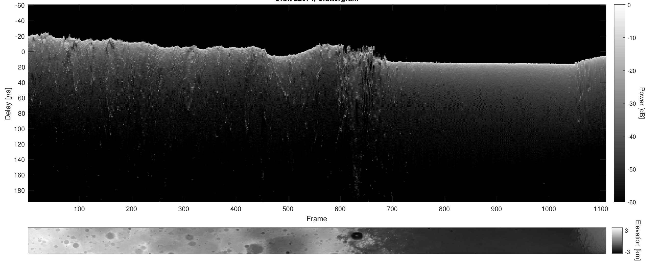
Orbit 22674, Cluttergram
