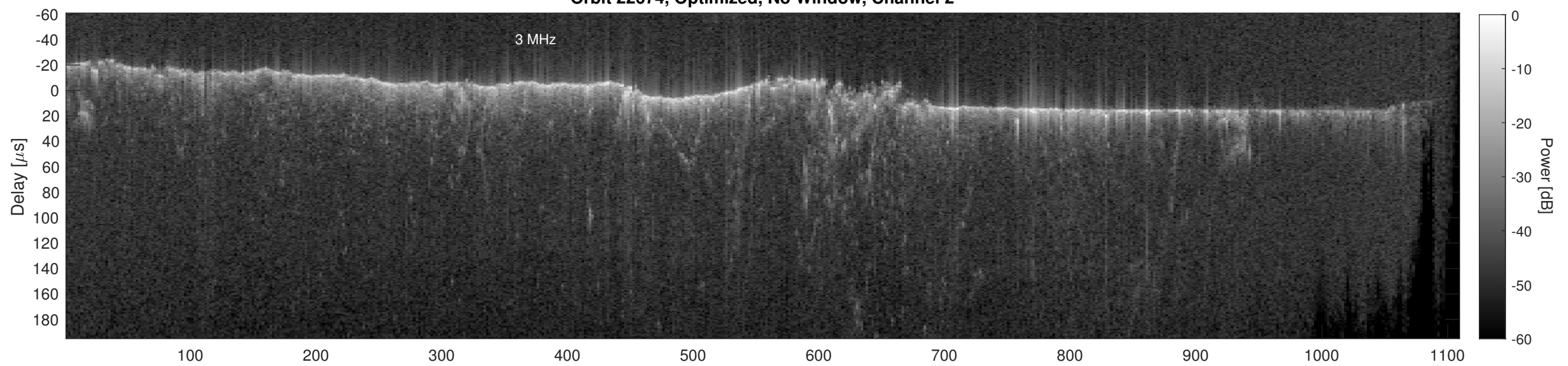
Orbit 22674, Cluttergram
