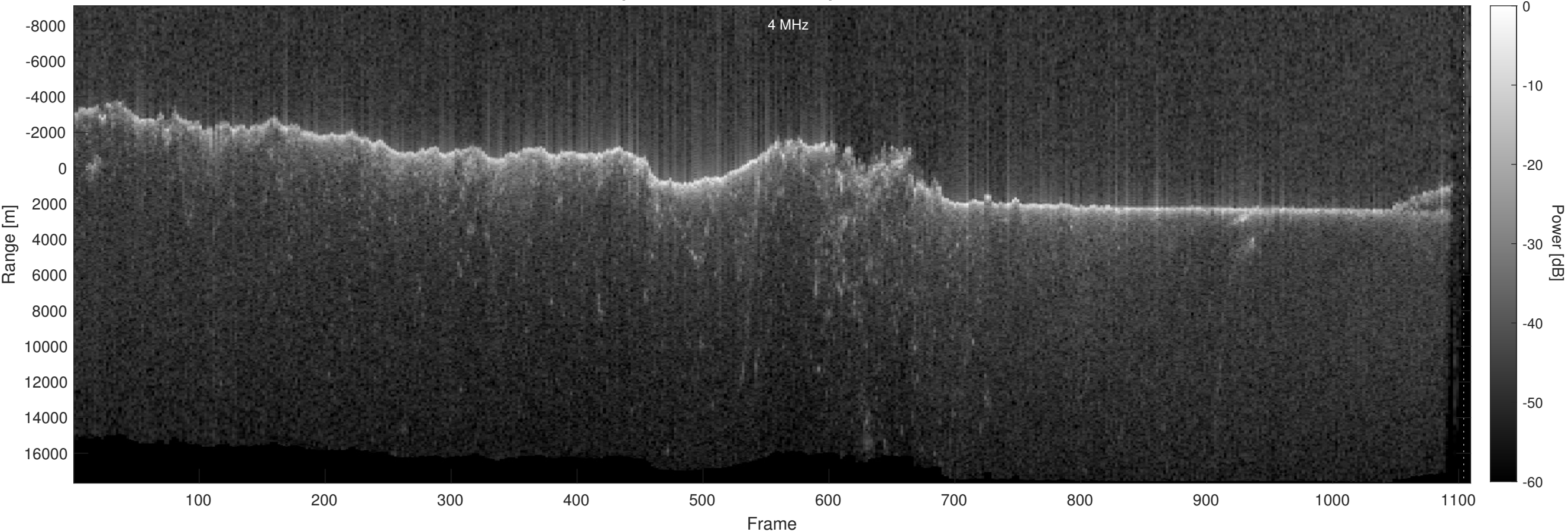
Orbit 22674, Optimized, No Window, Depth-Corrected, Channel 2
