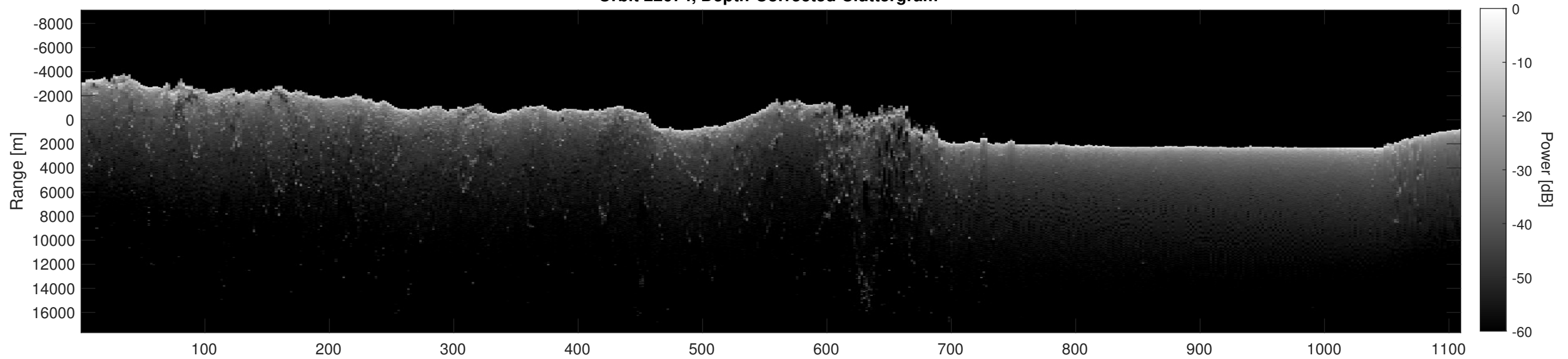
Orbit 22674, Depth-Corrected Cluttergram
