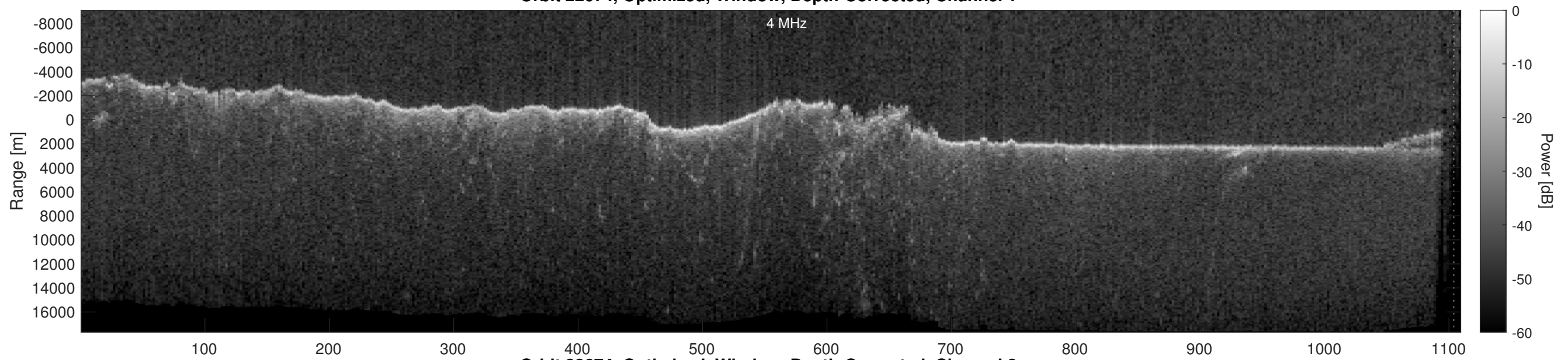
Orbit 22674, Optimized, Window, Depth-Corrected, Channel 2
