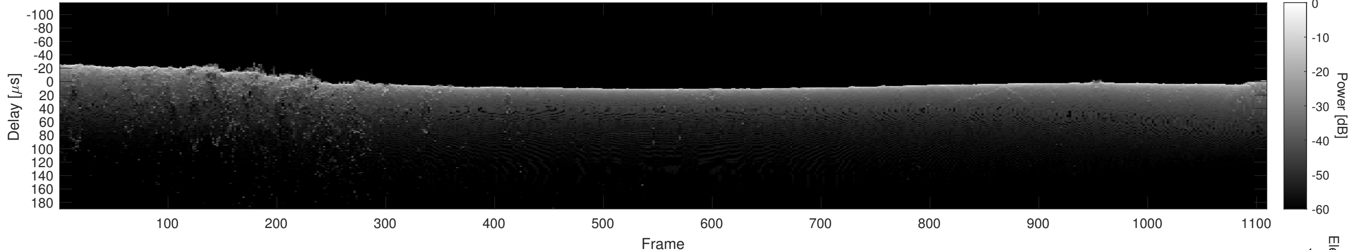
Orbit 22677, Cluttergram
