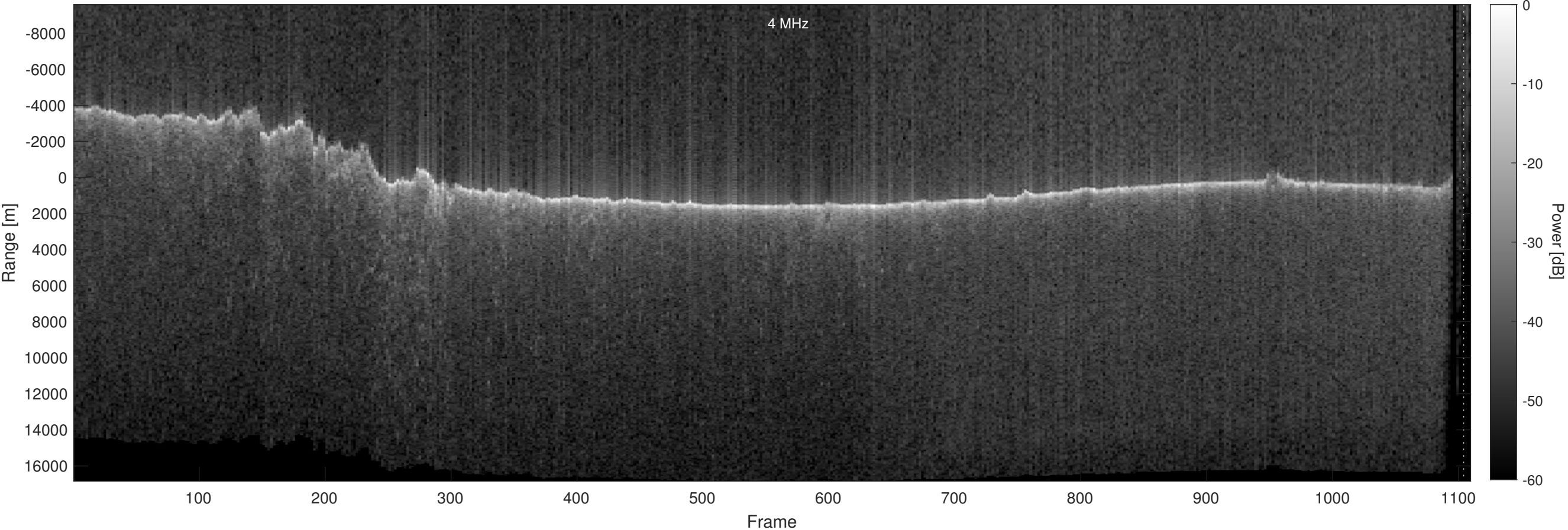
Orbit 22677, Optimized, No Window, Depth-Corrected, Channel 2
