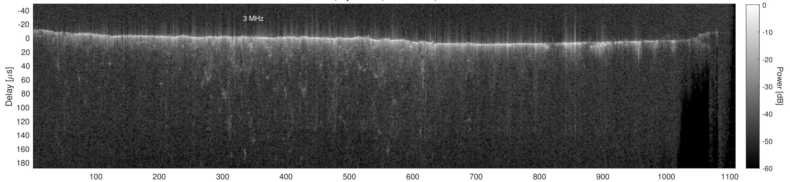
Orbit 22678, Cluttergram
