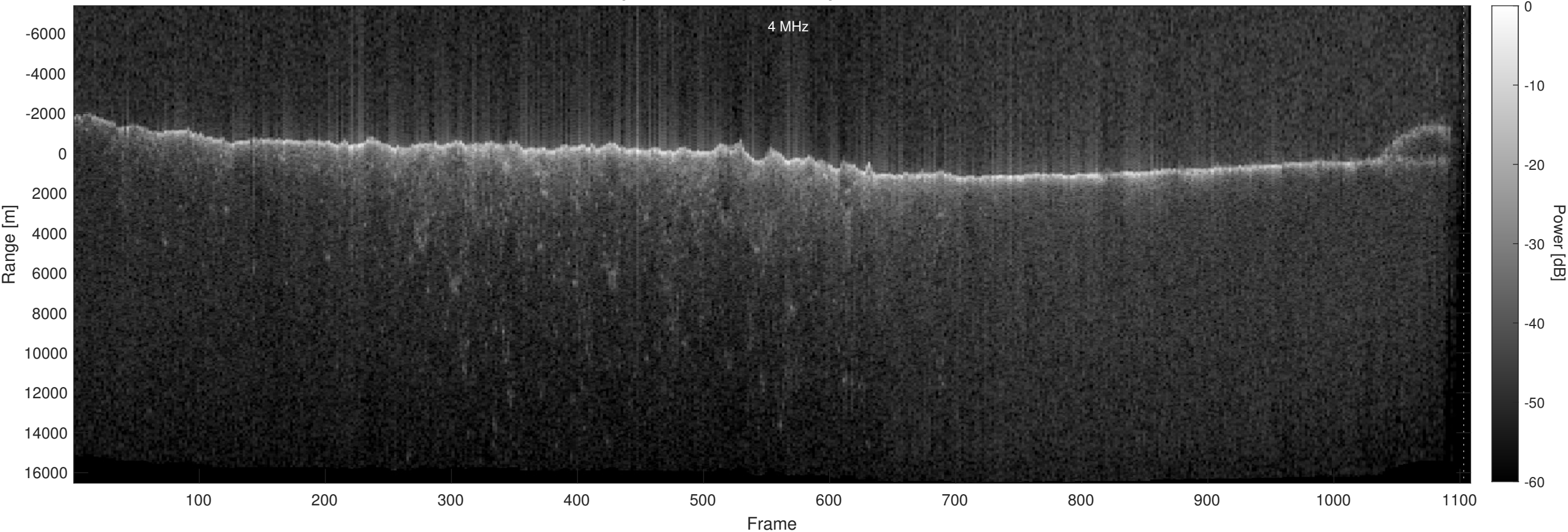
Orbit 22678, Optimized, No Window, Depth-Corrected, Channel 2
