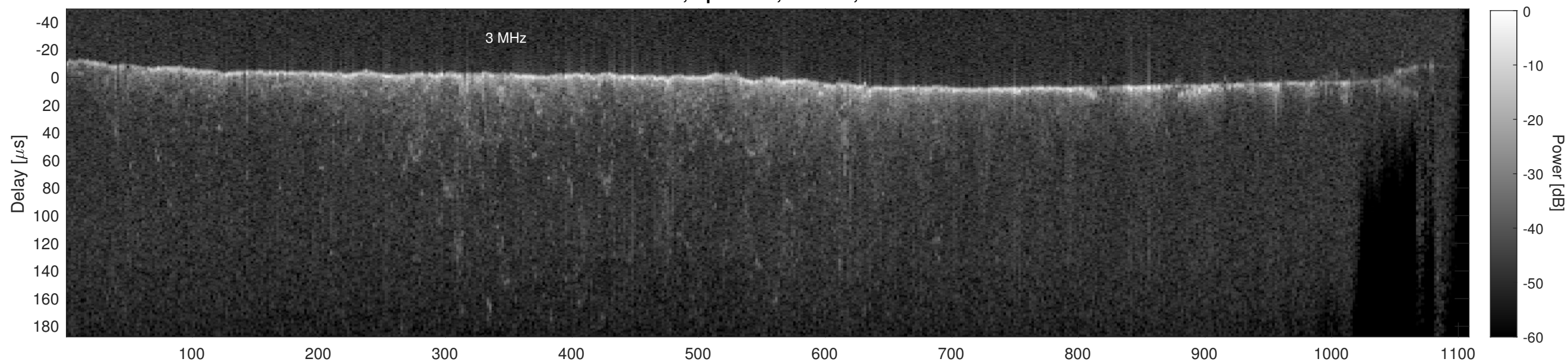
Orbit 22678, Cluttergram
