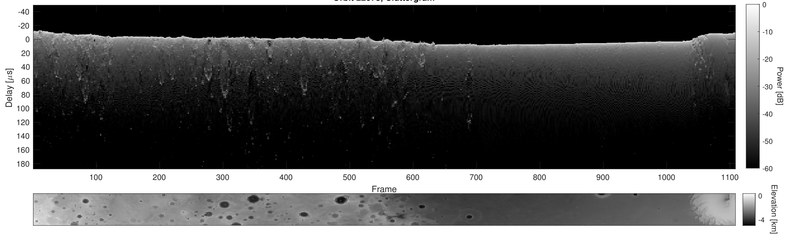
Orbit 22678, Cluttergram
