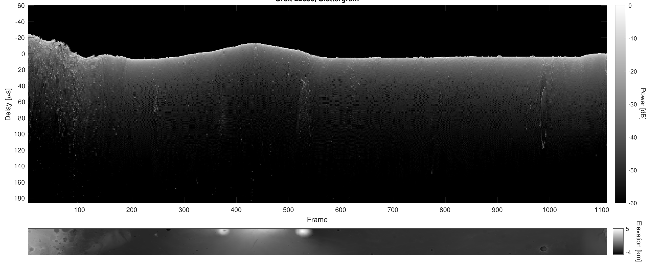
Orbit 22680, Cluttergram
