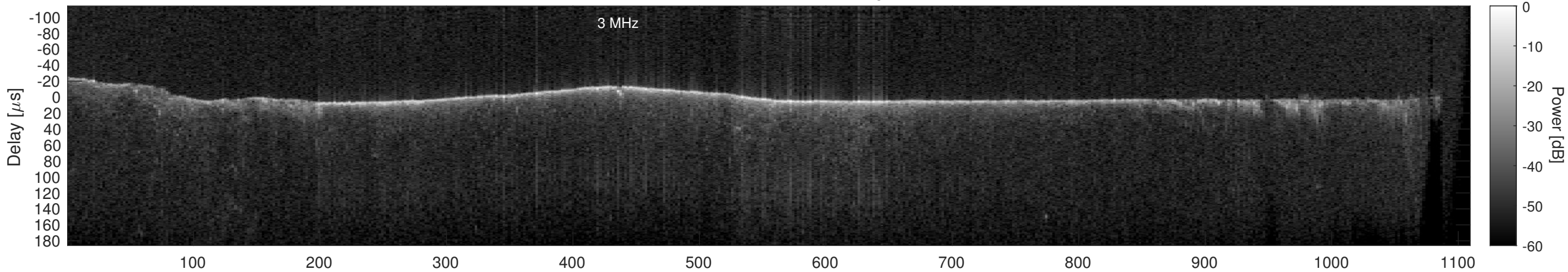
Orbit 22680, Cluttergram
