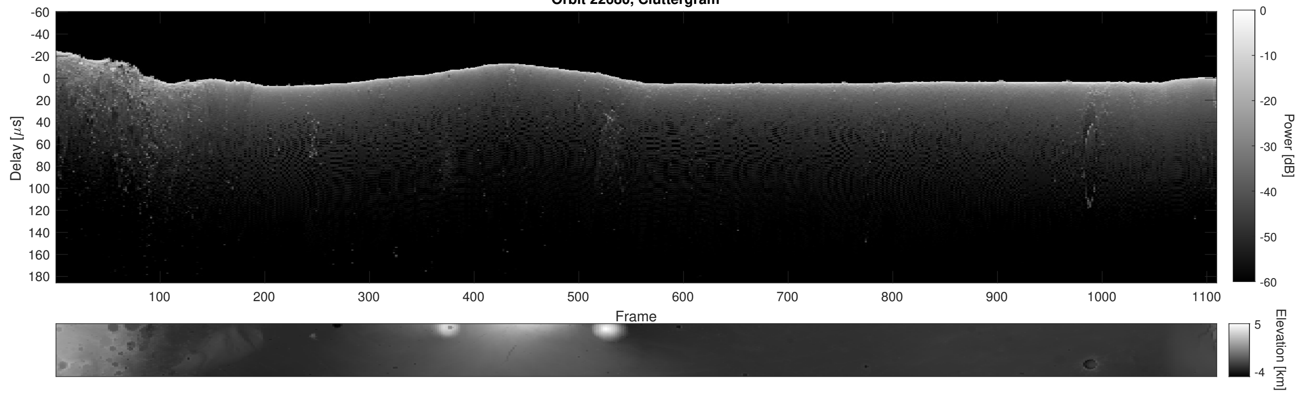
Orbit 22680, Cluttergram
