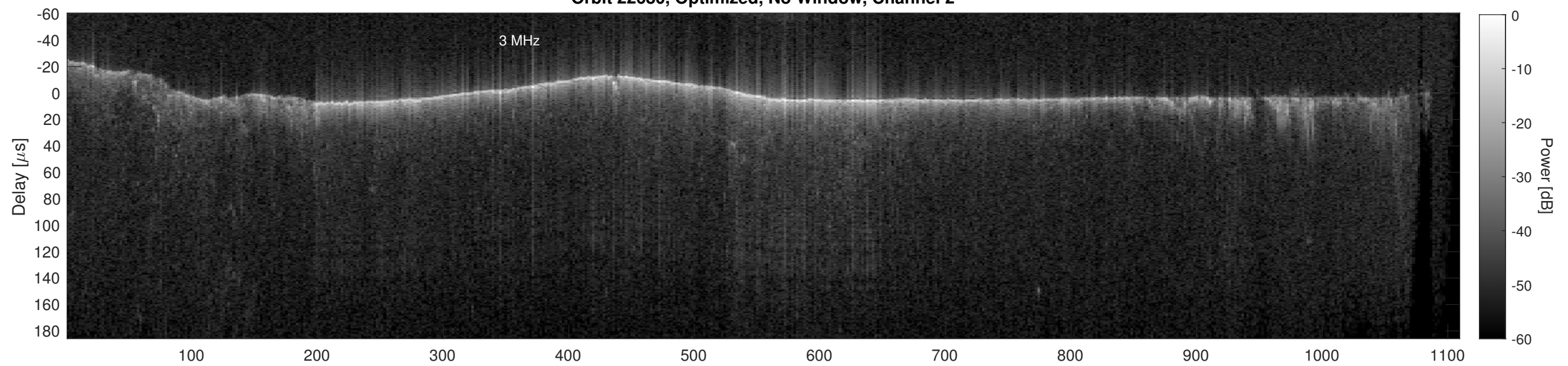
Orbit 22680, Cluttergram
