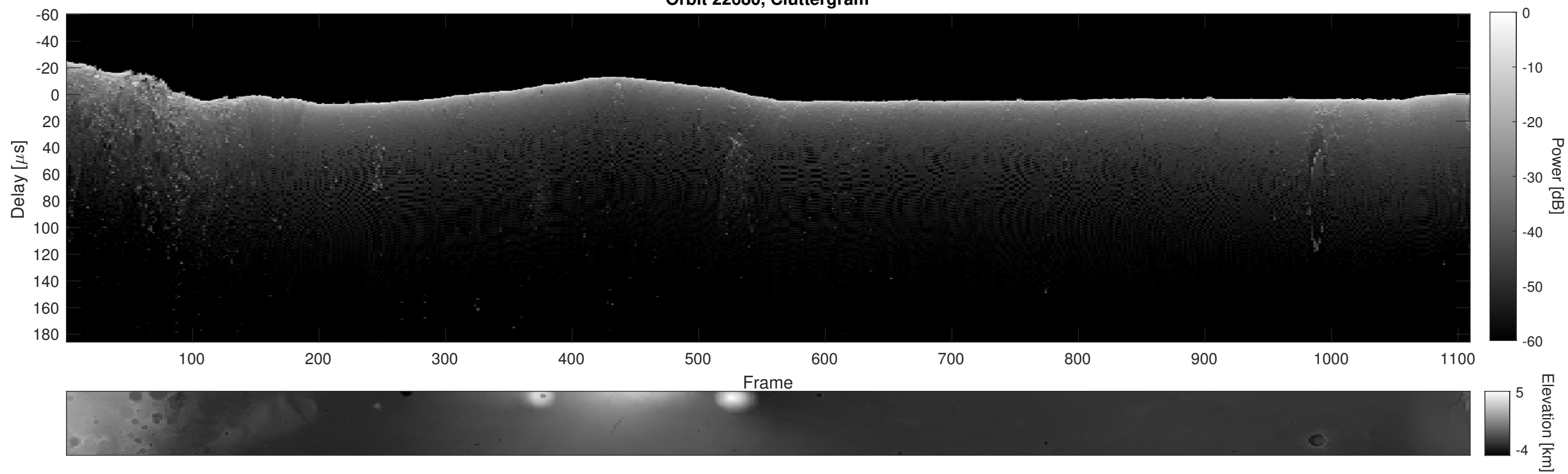
Orbit 22680, Cluttergram
