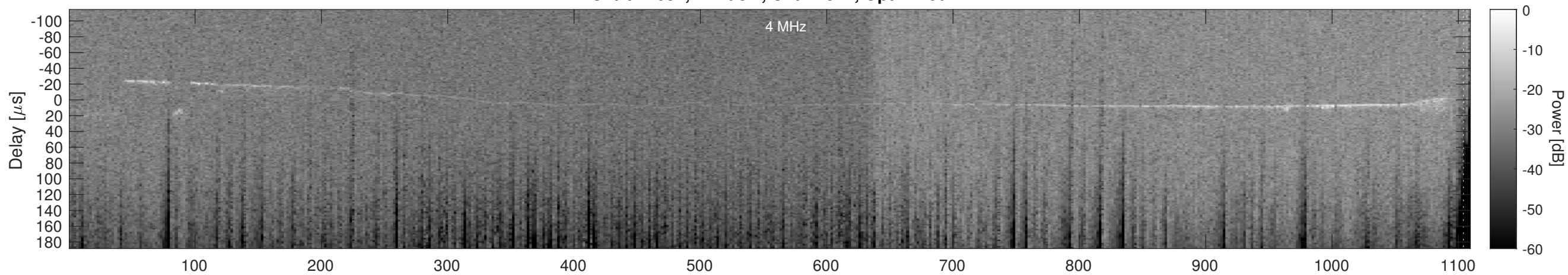
Orbit 22682, Cluttergram
