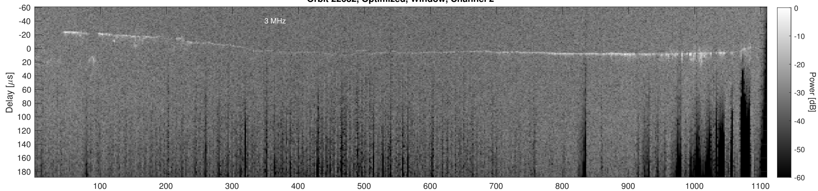
Orbit 22682, Cluttergram
