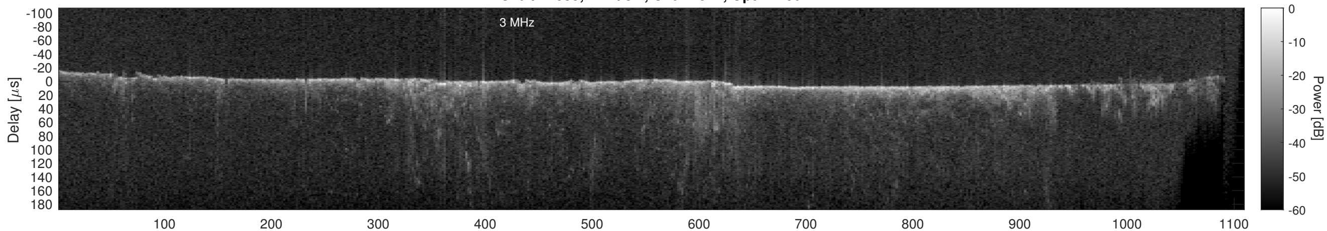
Orbit 22685, Cluttergram
