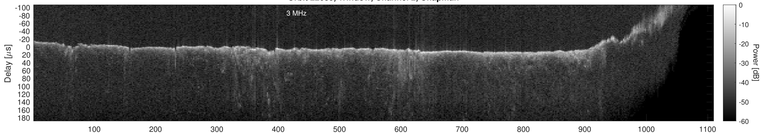
Orbit 22685, Window, Channel 2, Optimized
