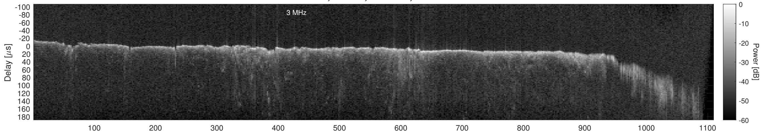
Orbit 22685, Window, Channel 2, Chapman
