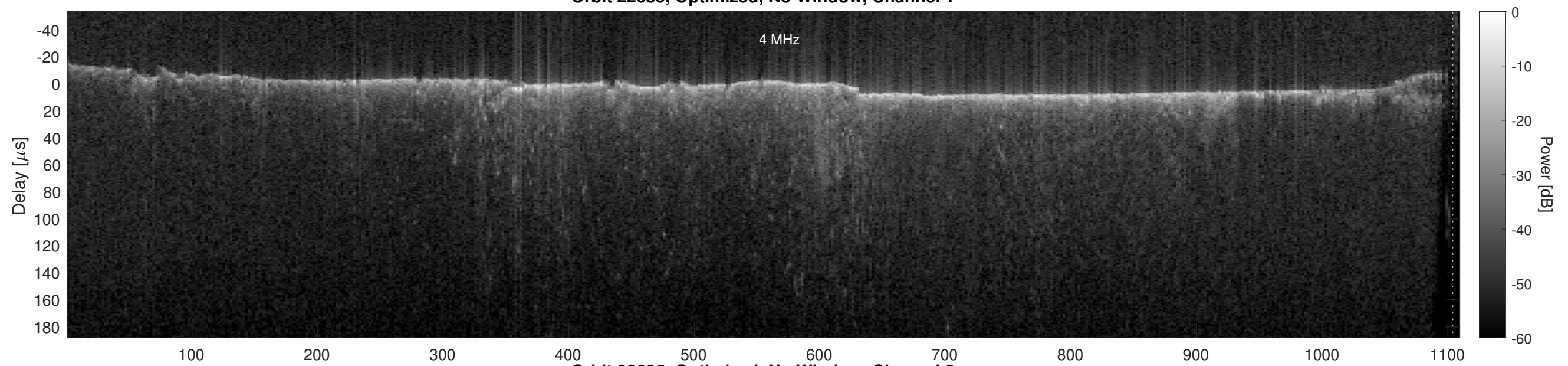
Orbit 22685, Optimized, No Window, Channel 2
