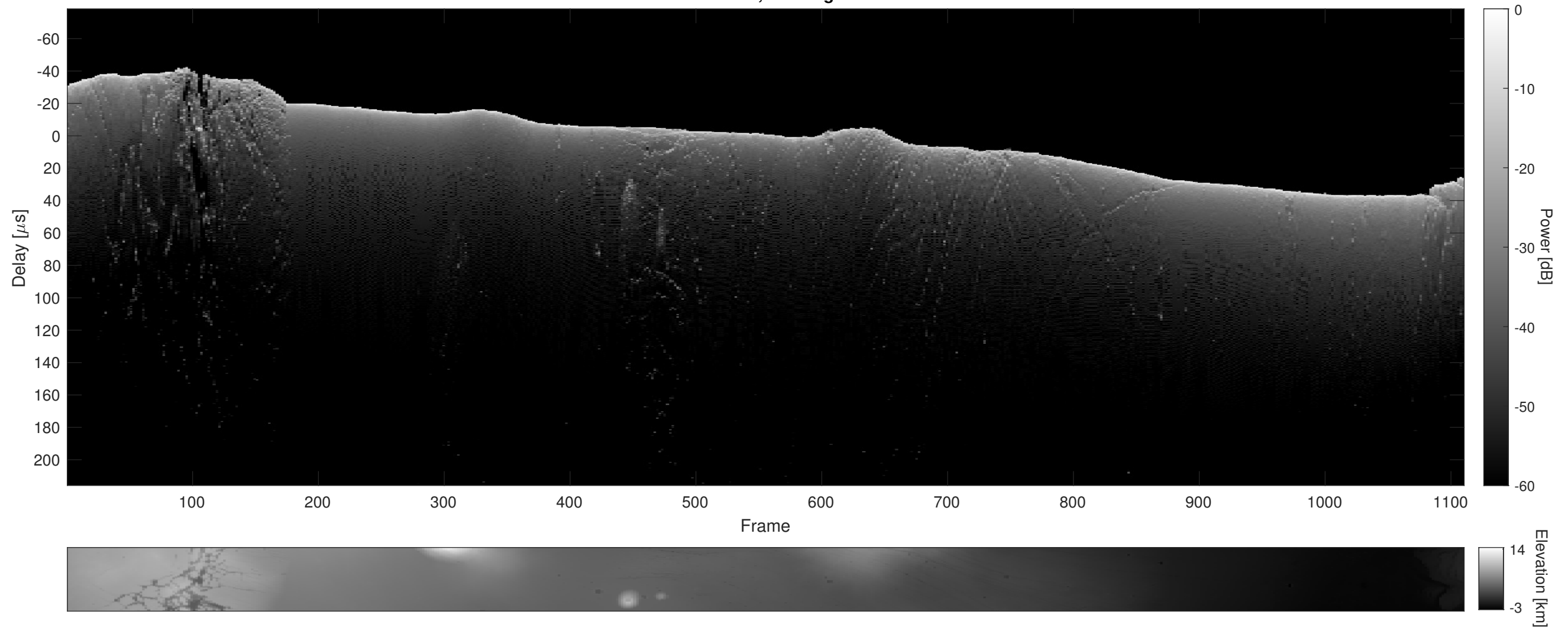
Orbit 22686, Cluttergram
