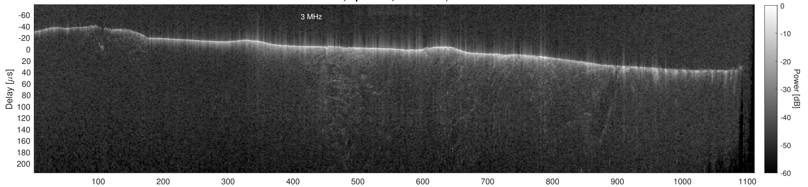
Orbit 22686, Cluttergram
