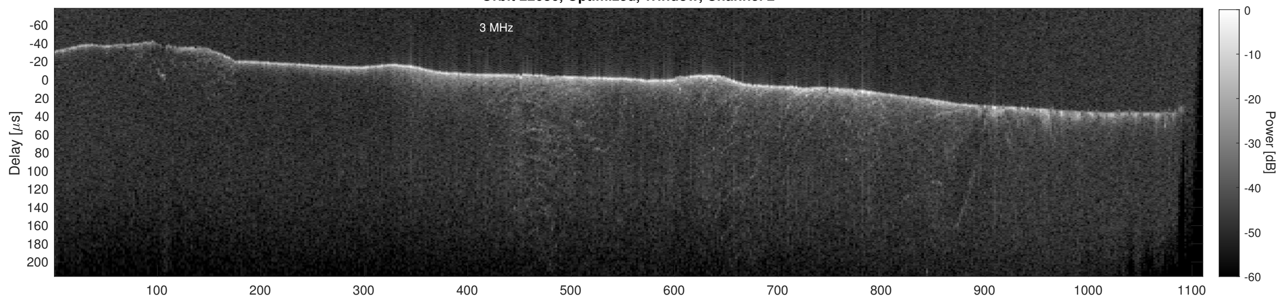
Orbit 22686, Cluttergram
