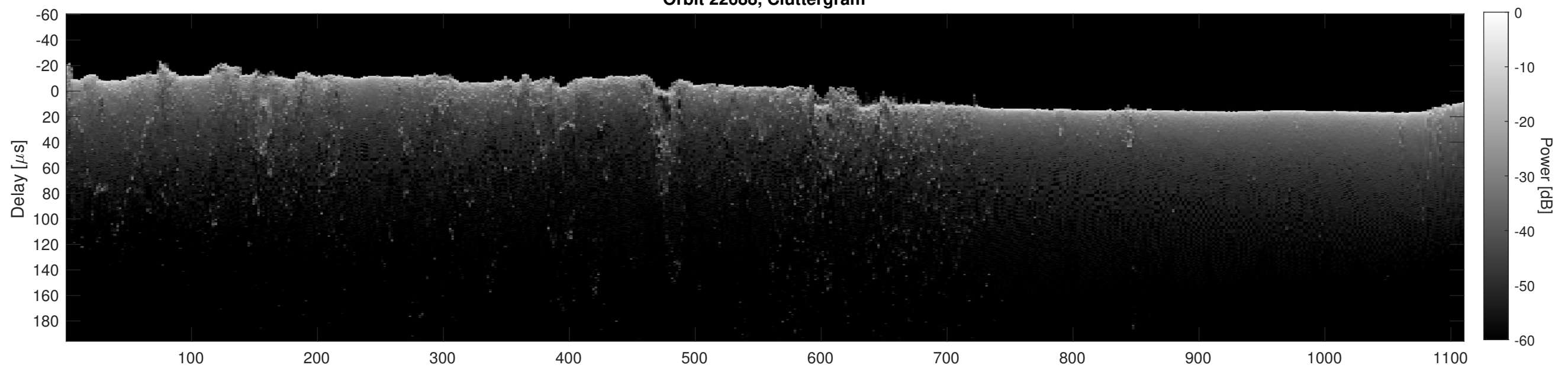
Orbit 22688, Cluttergram
