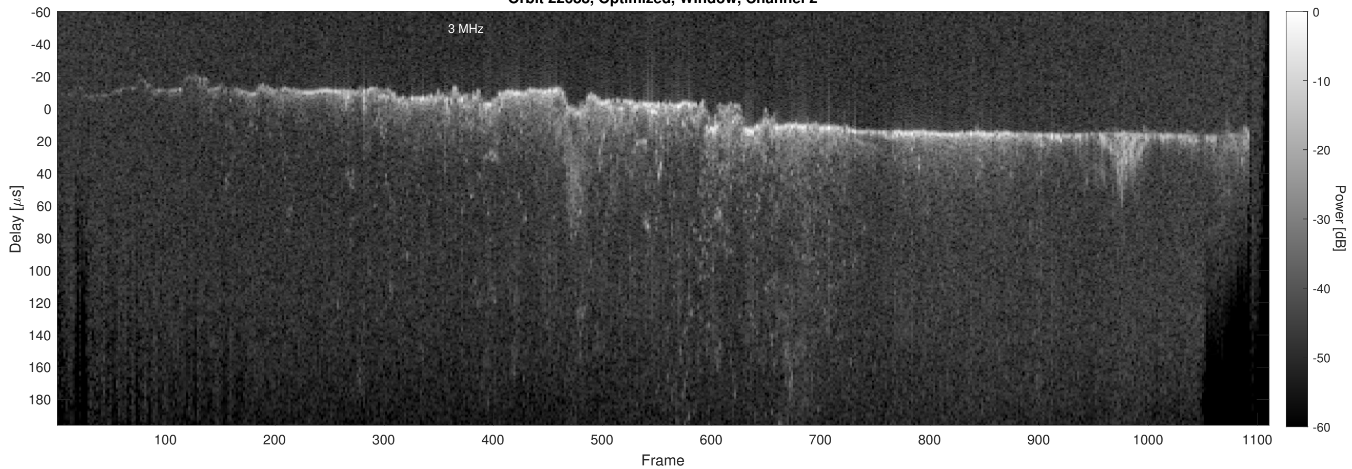
Orbit 22688, Optimized, Window, Channel 2
