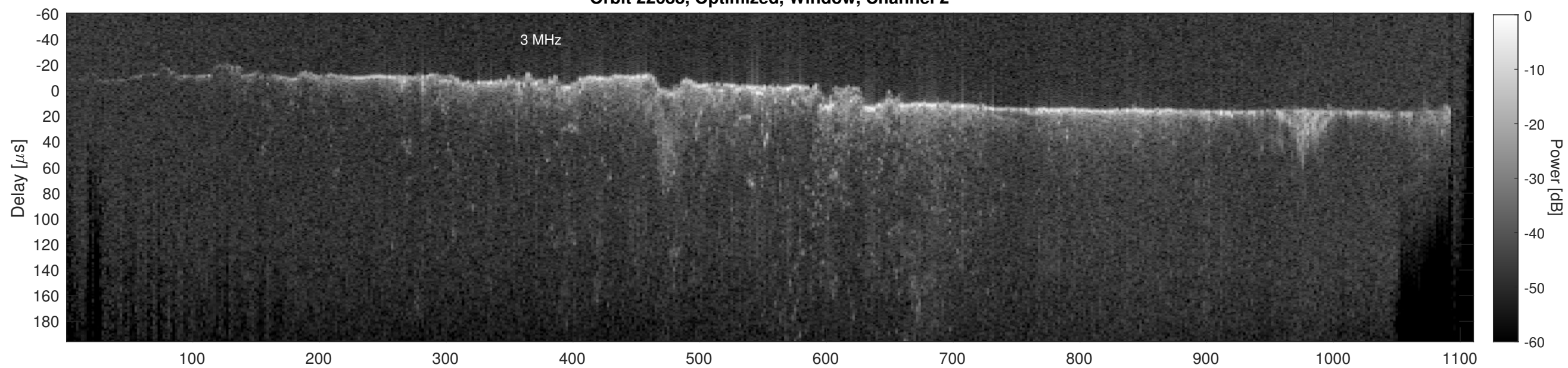
Orbit 22688, Cluttergram
