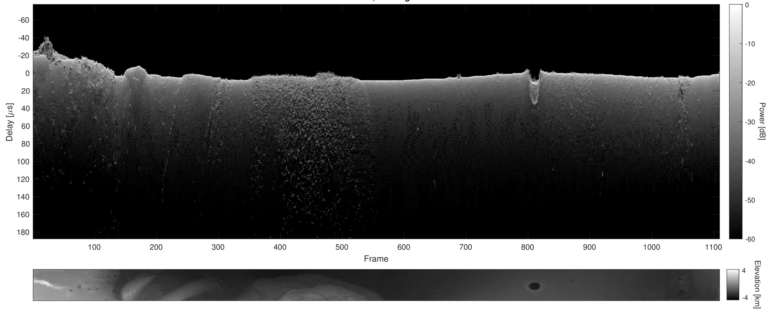
Orbit 22690, Cluttergram
