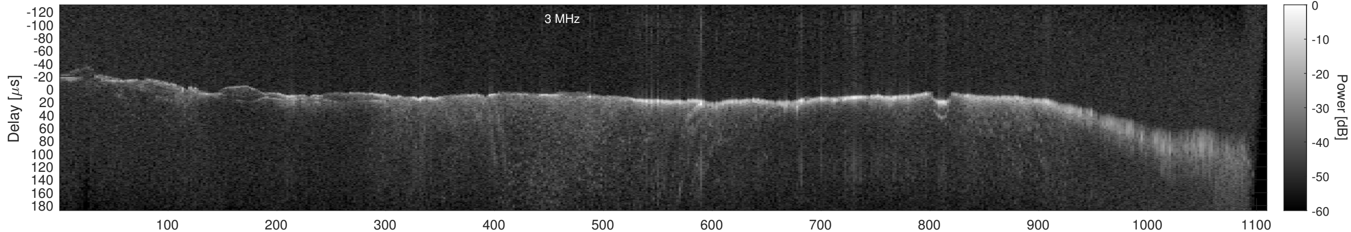
Orbit 22690, Window, Channel 2, Chapman
