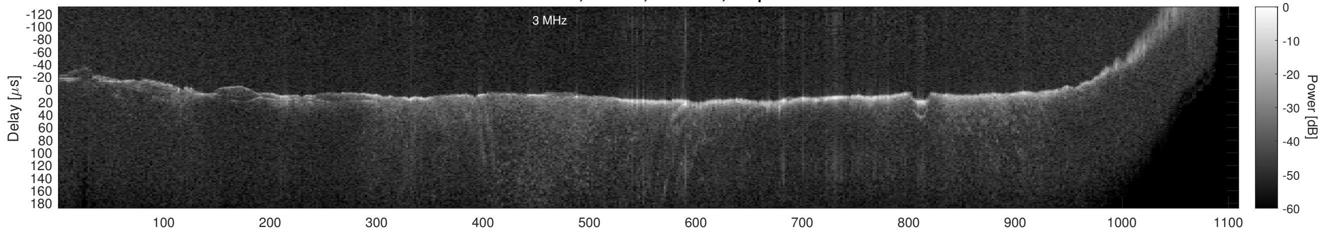
Orbit 22690, Window, Channel 2, Optimized
