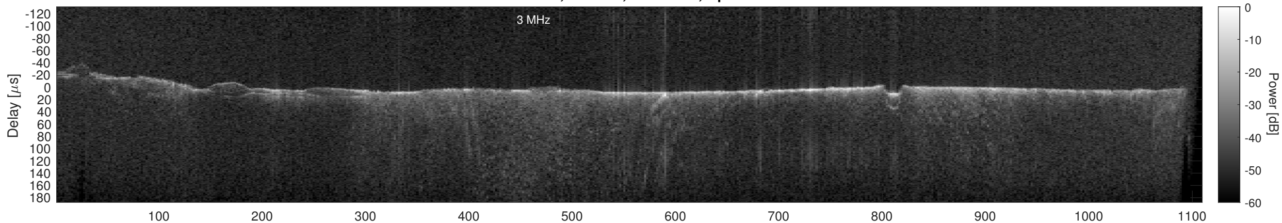
Orbit 22690, Cluttergram
