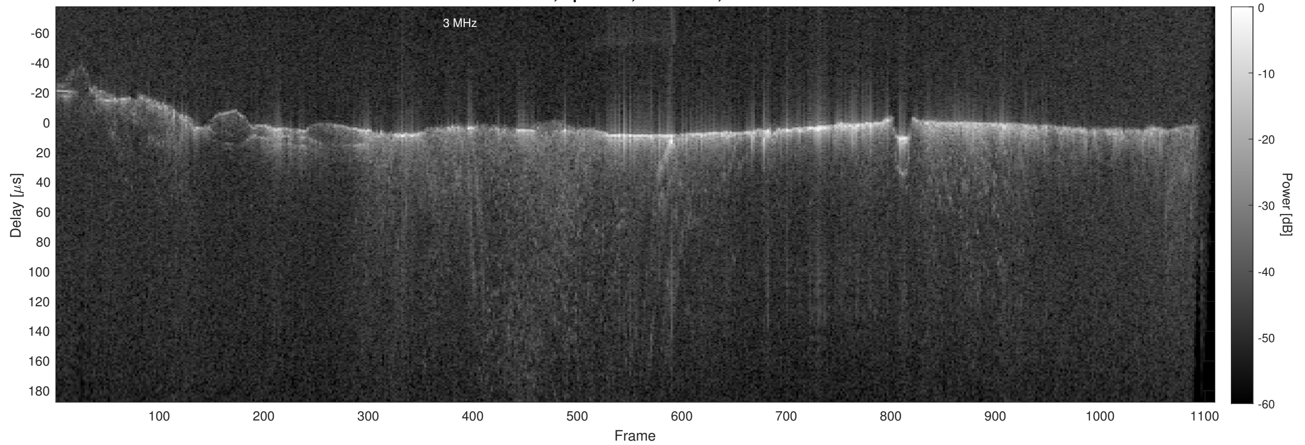
Orbit 22690, Optimized, No Window, Channel 2
