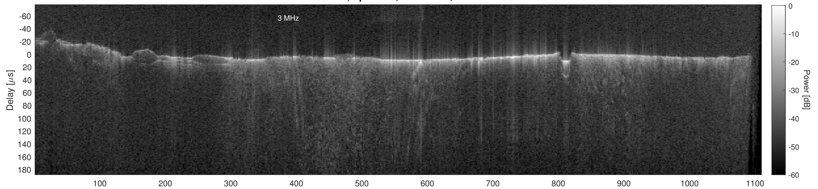
Orbit 22690, Cluttergram
