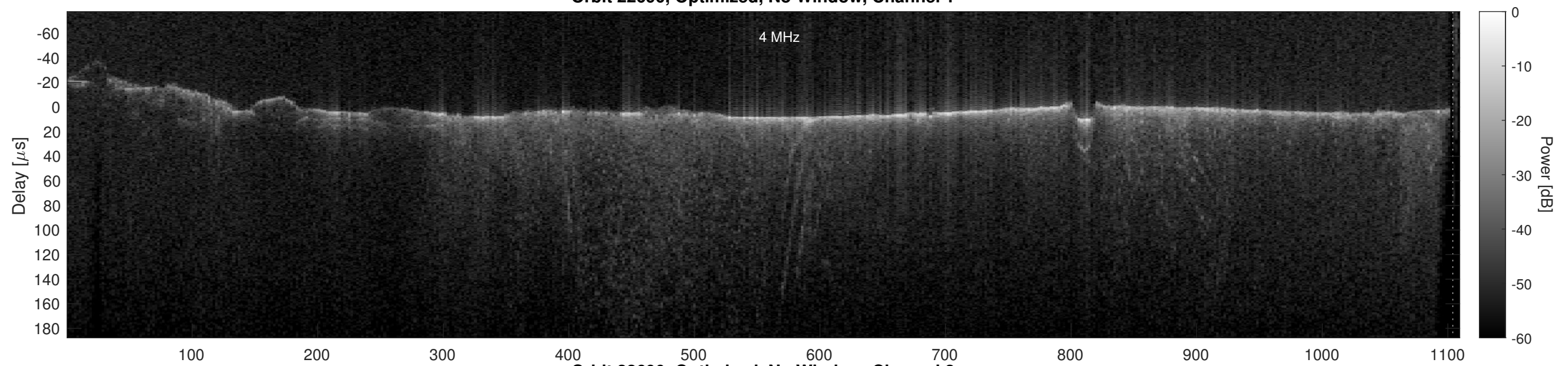
Orbit 22690, Optimized, No Window, Channel 2
