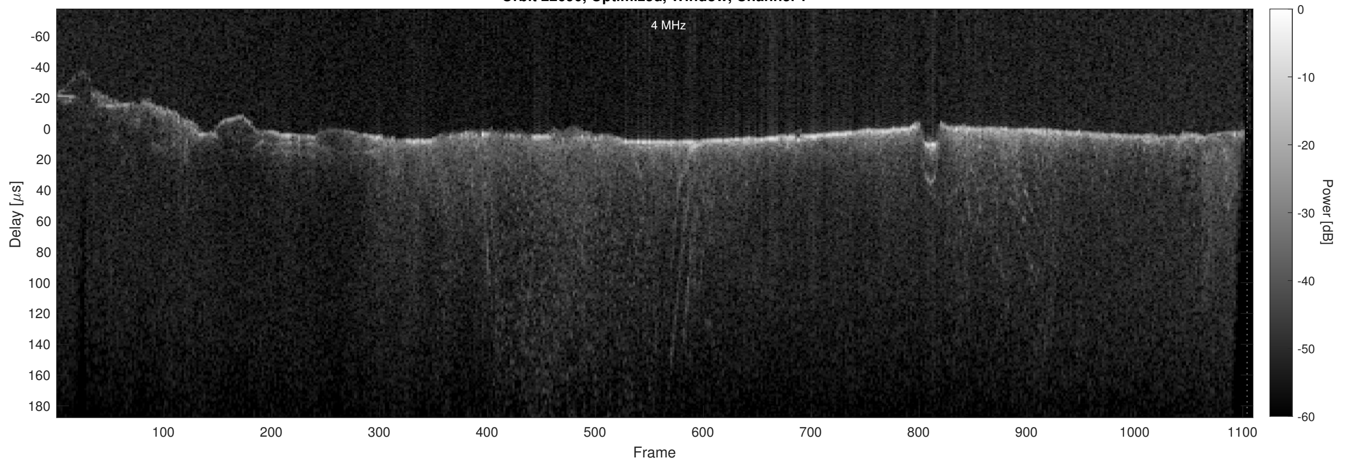
Orbit 22690, Optimized, Window, Channel 2
